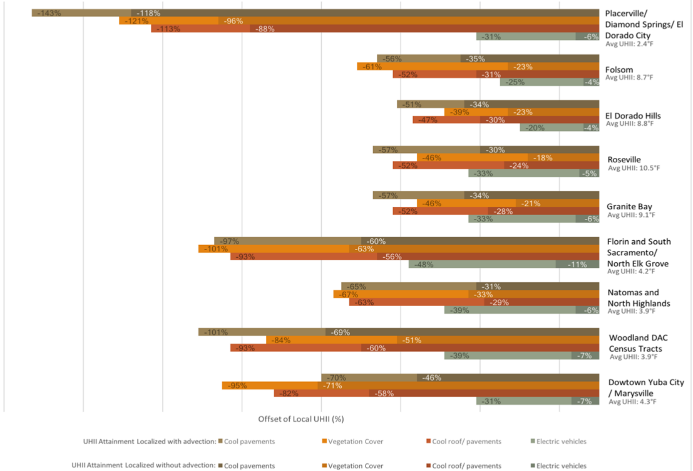
Figure 8. This graph shows the potential of local projects in mitigating the all-hours UHII in current climate and land use for different locations. The lower bar shows the percent reduction in UHII if the community implemented that measure alone (without advection), and the complete bar shows the percent reduction in UHII if the community and its upwind neighboring communities all implemented the same measure (with advection).
