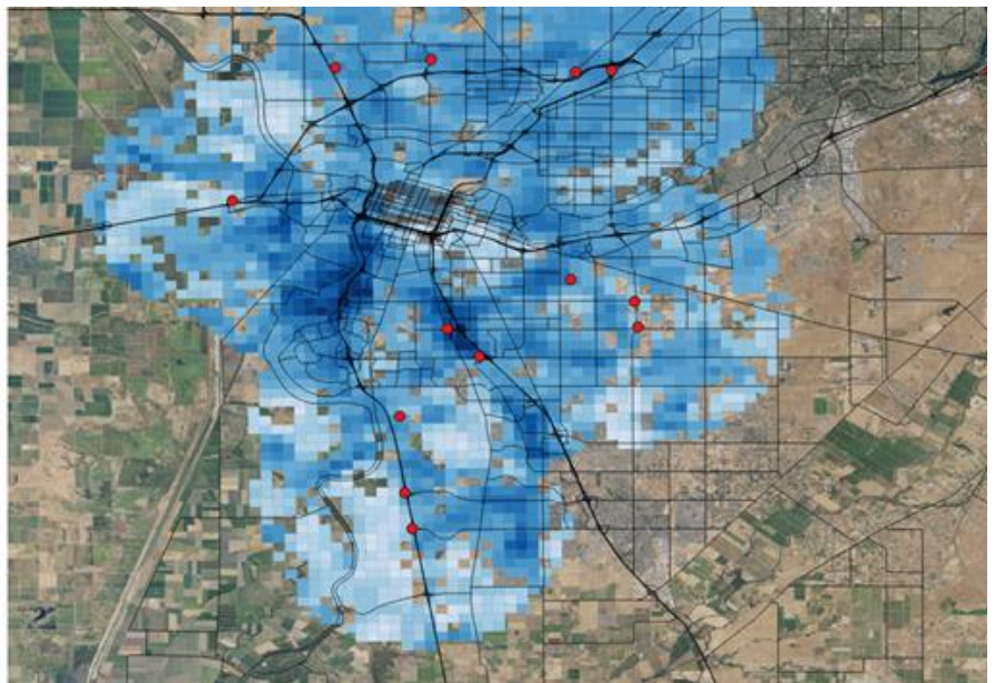
Figure 11. Average changes in surface temperature in central Sacramento at 5pm, assuming 25% vehicle electrification radiating out from proposed charging stations (red dots) in SMAQMD’s ZEV Readiness Plan. The modeled interval in this map is June 2015 and the maximum cooling is 5°F.
