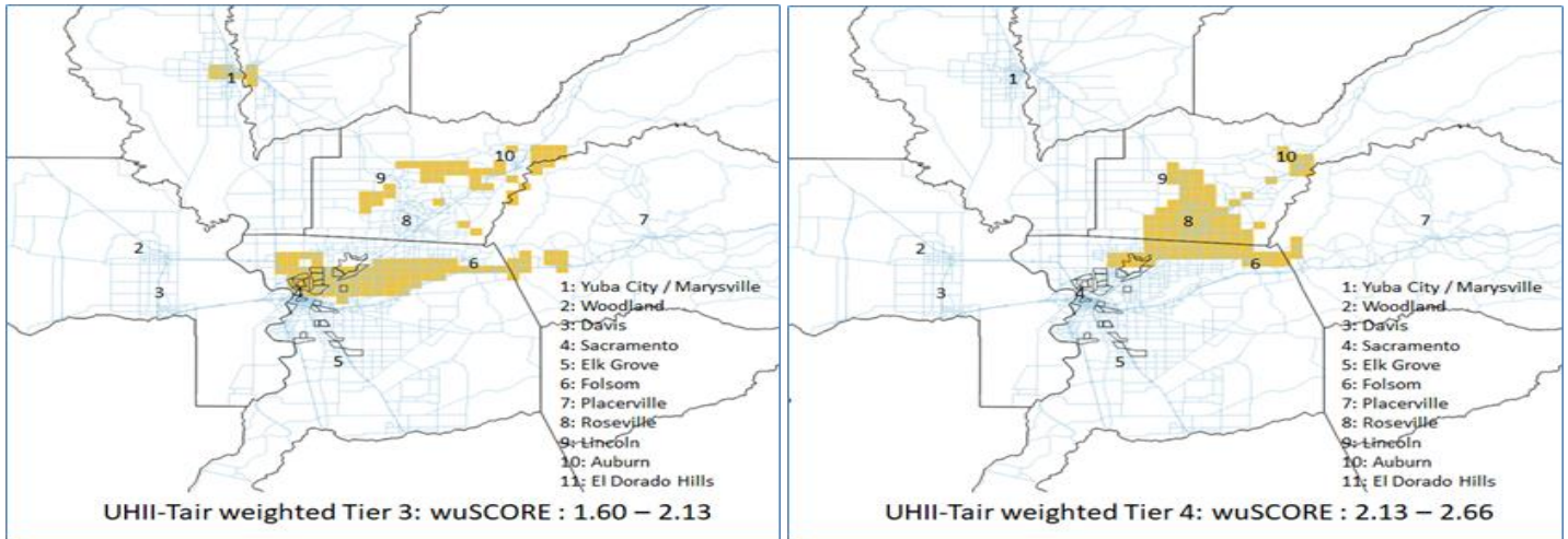
Figure 4. This UHI ranking score accounts for UHII as well as the absolute air temperature. Tier 4 (right) shows the highest priority areas for heat reduction under this scoring, and Tier 3 (left) shows the second highest priority areas.
