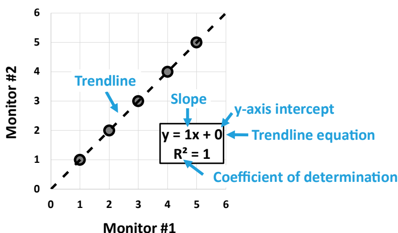
Figure 4-1. Linear regression explanation.
