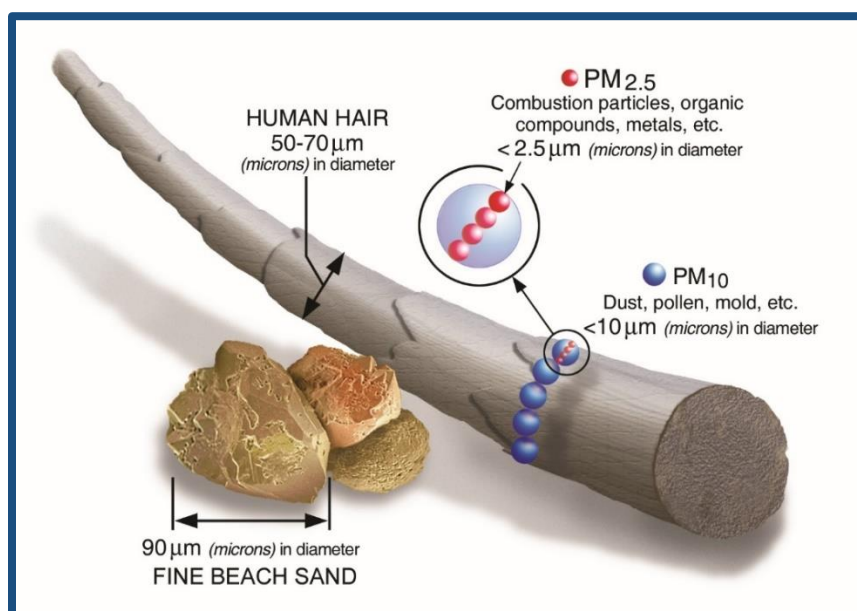
Figure 2-3. Particle size comparison.
