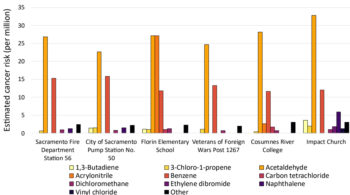
Figure 5-22. Estimated cancer risk from carcinogens measured by Phase 2 monitoring.
