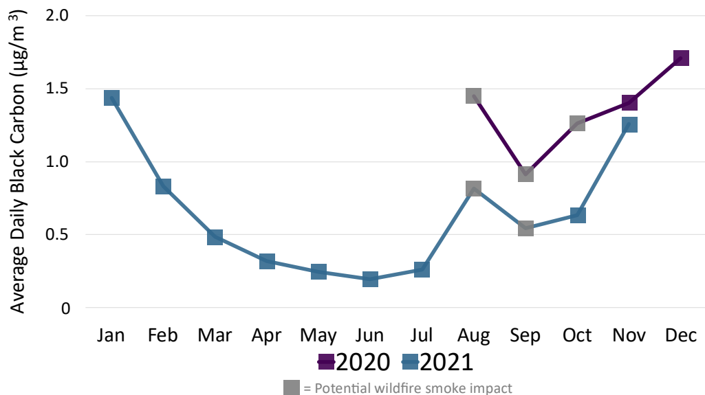
Figure 5-9. Monthly averages of Phase 2 monitoring black carbon levels.
