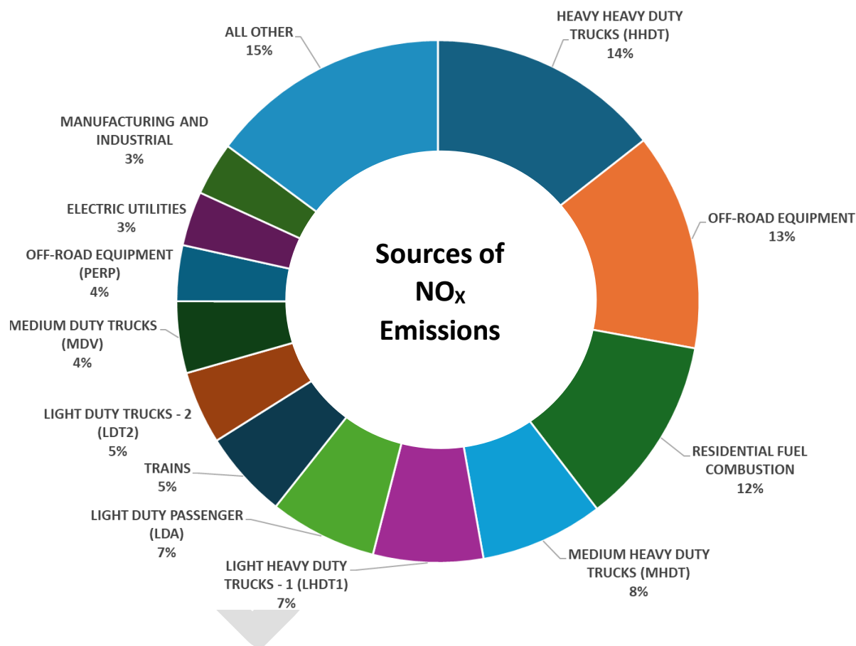
Figure 4-14 Sources of NO x in the South Sacramento-Florin Community based on the 2023 EI.
