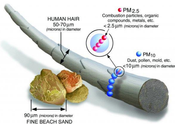
Figure 4-1 Particulate matter size comparisons. Source: U.S. EPA.
