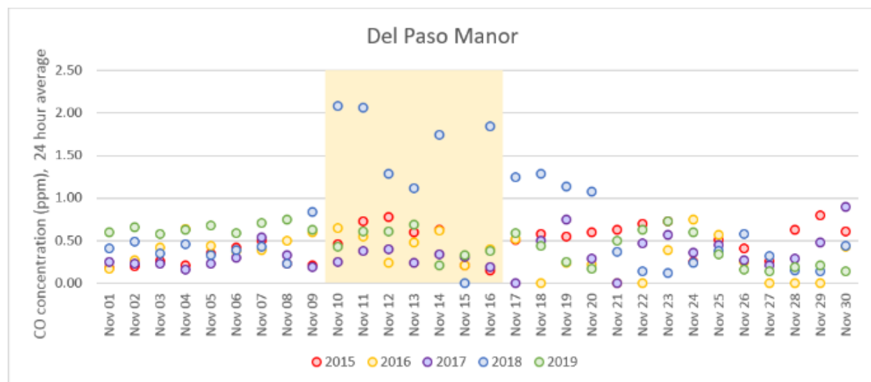
Figure 4-8(a-d) Carbon Monoxide, Black Carbon and Organic Carbon concentrations during November 2015 – 2019
