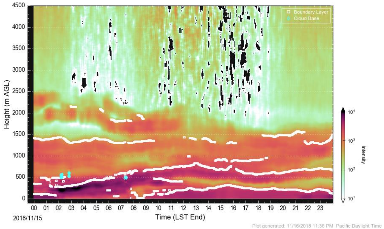
Figure 4-5 Ceilometer data collected for 11/15/2018
